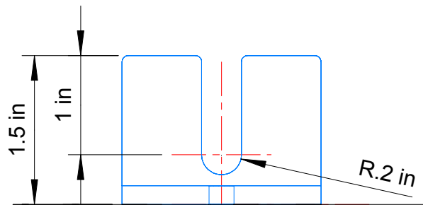
PART 2: CLAW Made from 1.5 x 1.5 x 3/16 aluminum angle
