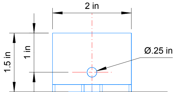
PART 2: CLAW Made from 1.5 x 1.5 x 3/16 aluminum angle
